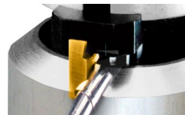
37.5° bevel x 0.125" land 6" schedule 160
